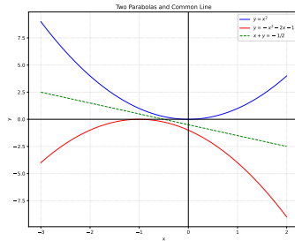
Fig. 1.1.1.1. The two parabolas and the common-chord line x + y = -\frac{1}{2}
