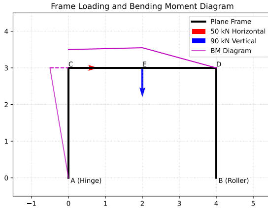
Fig. 1.1.10.1. Frame loading and bending moment diagram
