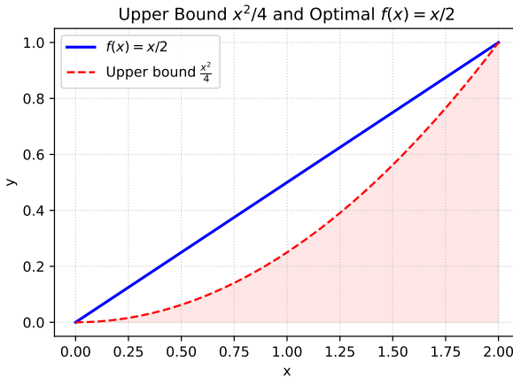
Fig. 1.1.7.1. The integrand attains its upper bound \frac{x^2}{4} only for f(x) = \frac{x}{2}
