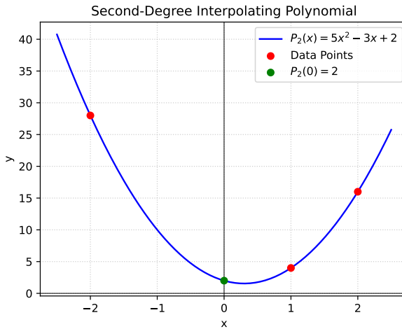
Fig. 1.1.12.1. Interpolating polynomial through the given points
