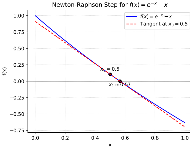
Fig. 1.1.11.1. One Newton-Raphson step for f(x) = e^{-x} - x from x_0 = 0.5
