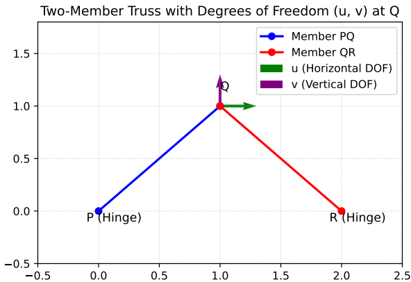
Fig. 1.1.9.1. Two-member truss with degrees of freedom u, v at Q
