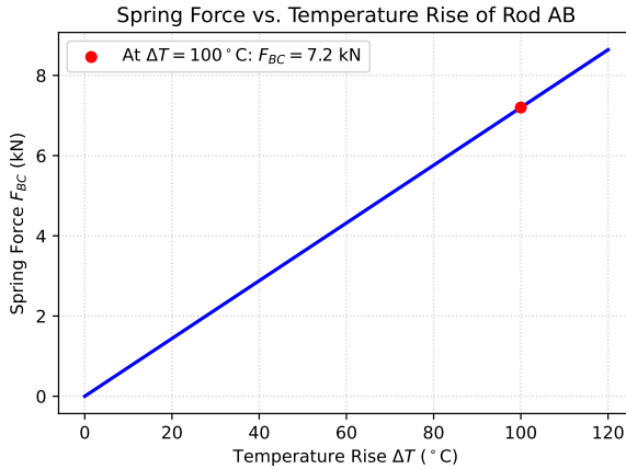
Fig. 1.1.14.1. Rod AB connected in series with spring BC under thermal loading
