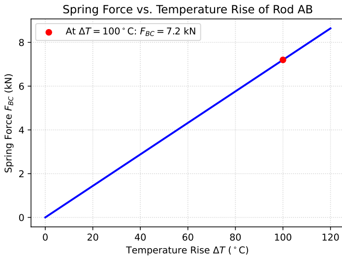
Fig. 1.1.19.1. Rod AB connected in series with spring BC under thermal loading
