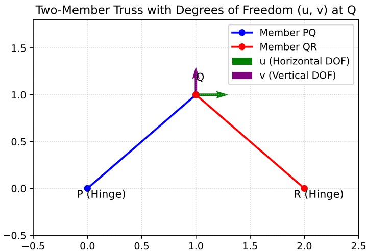
Fig. 1.1.14.1. Two-member truss with degrees of freedom u, v at Q
