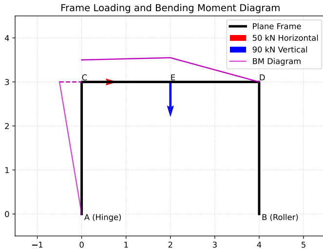
Fig. 1.1.15.1. Frame loading and bending moment diagram
