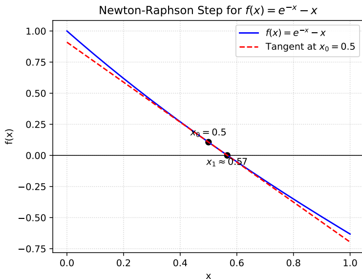
Fig. 1.1.16.1. One Newton-Raphson step for f(x) = e^{-x} - x from x_0 = 0.5
