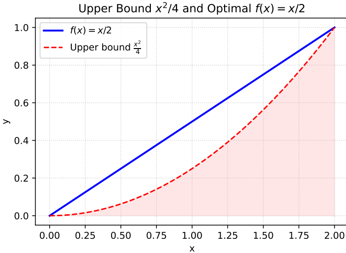
Fig. 1.1.12.1. The integrand attains its upper bound \frac{x^2}{4} only for f(x) = \frac{x}{2}
