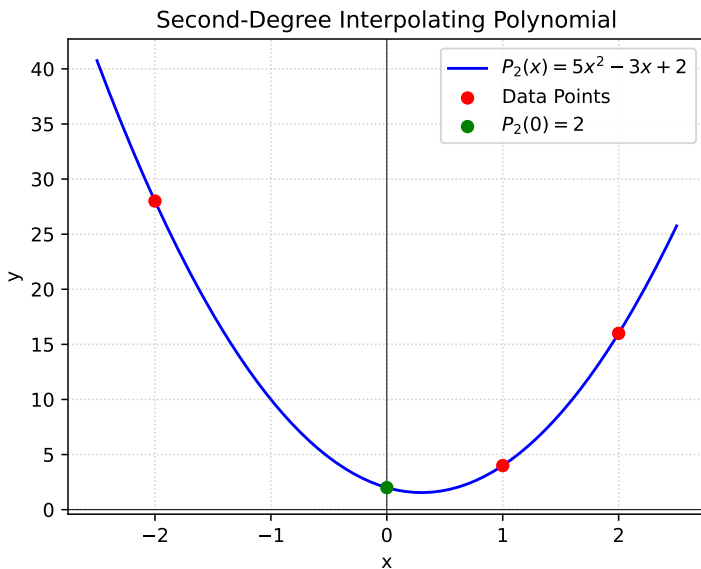
Fig. 1.1.17.1. Interpolating polynomial through the given points
