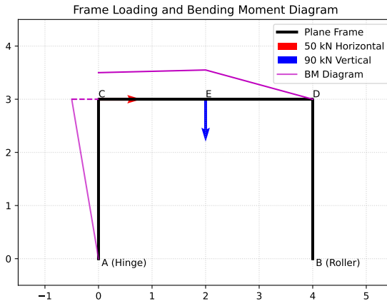
Fig. 1.1.15.1. Frame loading and bending moment diagram
