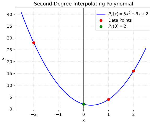
Fig. 1.1.17.1. Interpolating polynomial through the given points
