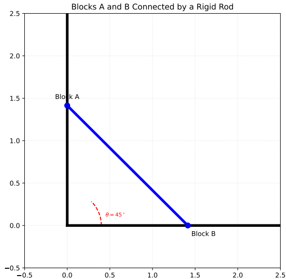
Fig. 1.1.16.1. Blocks A and B connected by a rigid rod at \theta = 45^\circ
