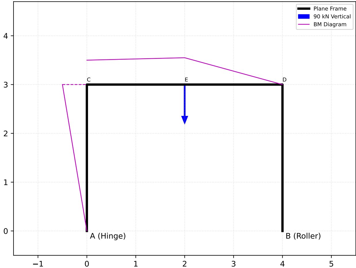
Frame Loading and Bending Moment Diagram
