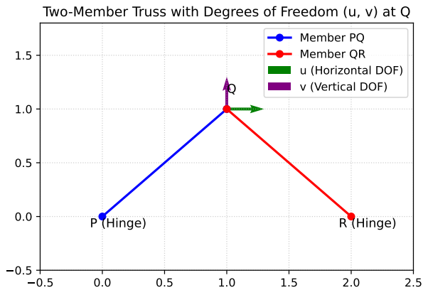
Fig. 1.1.11.1. Two-member truss with degrees of freedom u , v at Q
