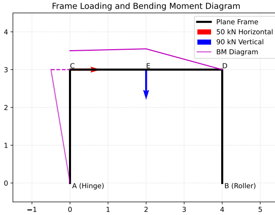
Fig. 4.1. Frame loading and bending moment diagram
