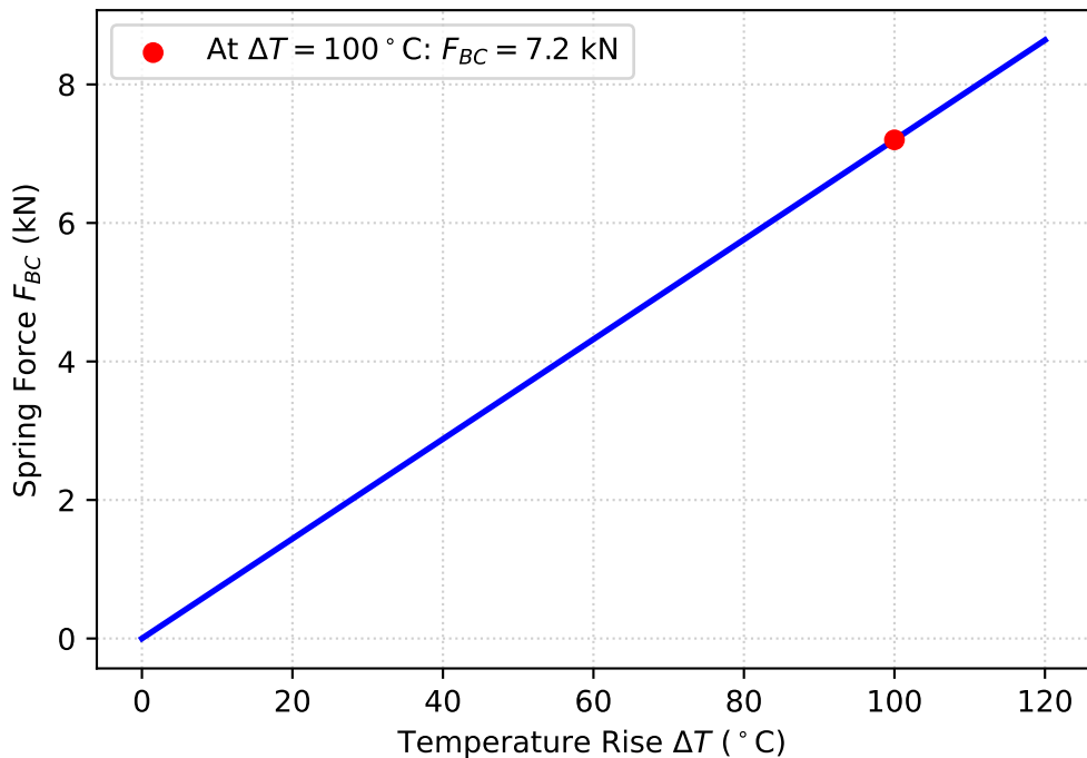
Spring Force vs. Temperature Rise of Rod AB
