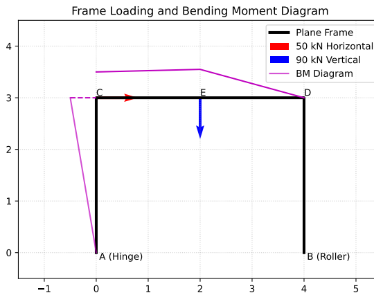
Fig. 1.1.12.1. Frame loading and bending moment diagram
