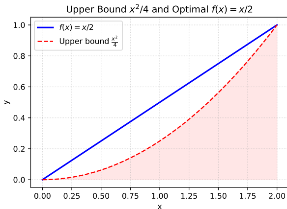
Fig. 1.1.9.1. The integrand attains its upper bound \frac{x^2}{4} only for f(x) = \frac{x}{2}
