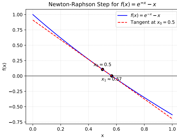
Fig. 1.1.13.1. One Newton-Raphson step for f(x) = e^{-x} - x from x_0 = 0.5
