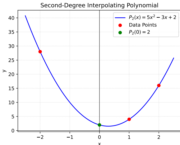
Fig. 1.1.13.1. Interpolating polynomial through the given points
