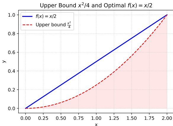
Fig. 1.1.11.1. The integrand attains its upper bound \frac{x^2}{4} only for f(x) = \frac{x}{2}
