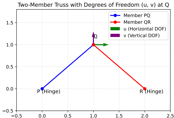
Fig. 1.1.10.1. Two-member truss with degrees of freedom u, v at Q
