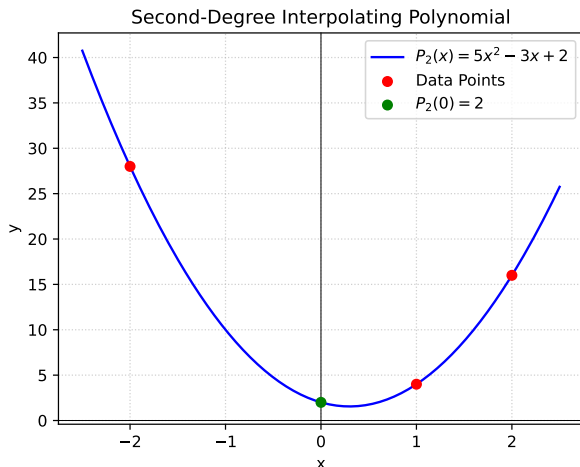
Fig. 1.1.15.1. Interpolating polynomial through the given points
