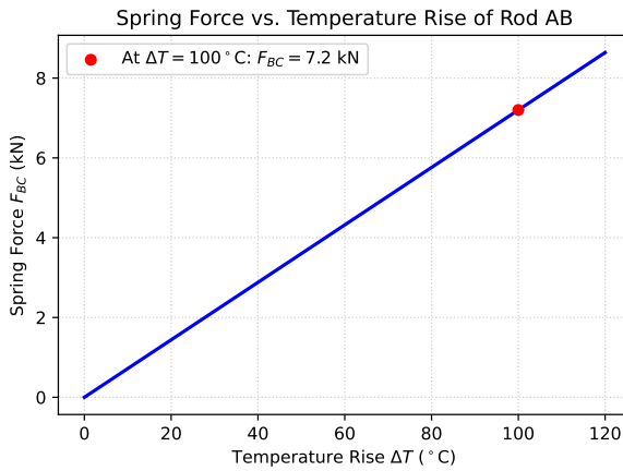
Fig. 1.1.17.1. Rod AB connected in series with spring BC under thermal loading
