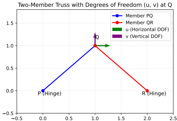
Fig. 1.1.12.1. Two-member truss with degrees of freedom u, v at Q
