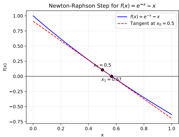
Fig. 1.1.14.1. One Newton-Raphson step for f(x) = e^{-x} - x from x_0 = 0.5
