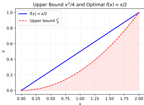
Fig. 1.1.10.1. The integrand attains its upper bound \frac{x^2}{4} only for f(x) = \frac{x}{2}
