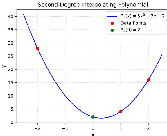
Fig. 1.1.15.1. Interpolating polynomial through the given points
