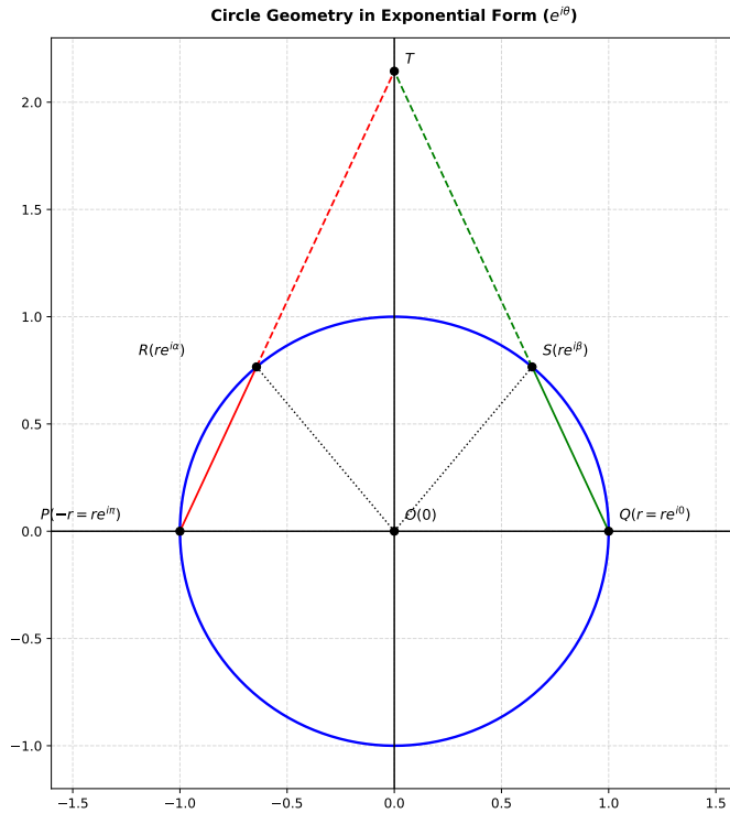
Fig. 1.1.2.1. Circle with diameter PQ , \angle ROS = 80^\circ and \angle RTS = 50^\circ
