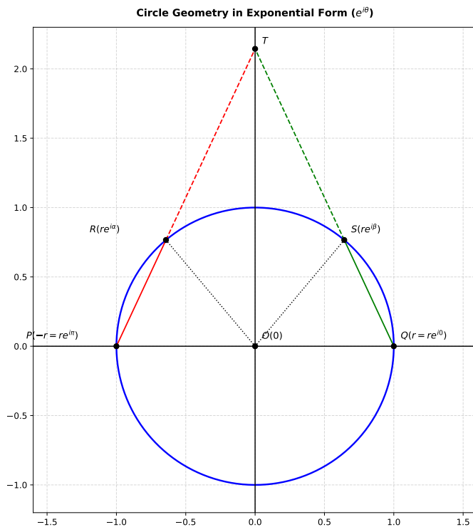
Fig. 1.1.3.2. Circle with diameter PQ , \angle ROS = 80^\circ and \angle RTS = 50^\circ
