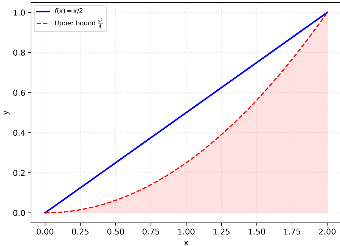
Upper Bound x^2/4 and Optimal f(x) = x/2
