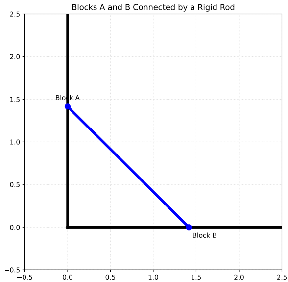
Fig. 14.3. Blocks A and B connected by a rigid rod at \theta = 45^\circ
