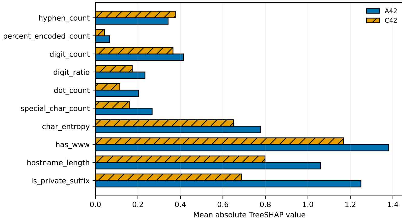
M2 engineered-feature global attribution (largest A42/C42 shifts)
