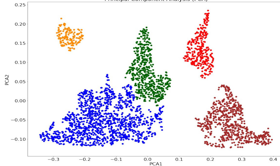
Principal Component Analysis (PCA)
