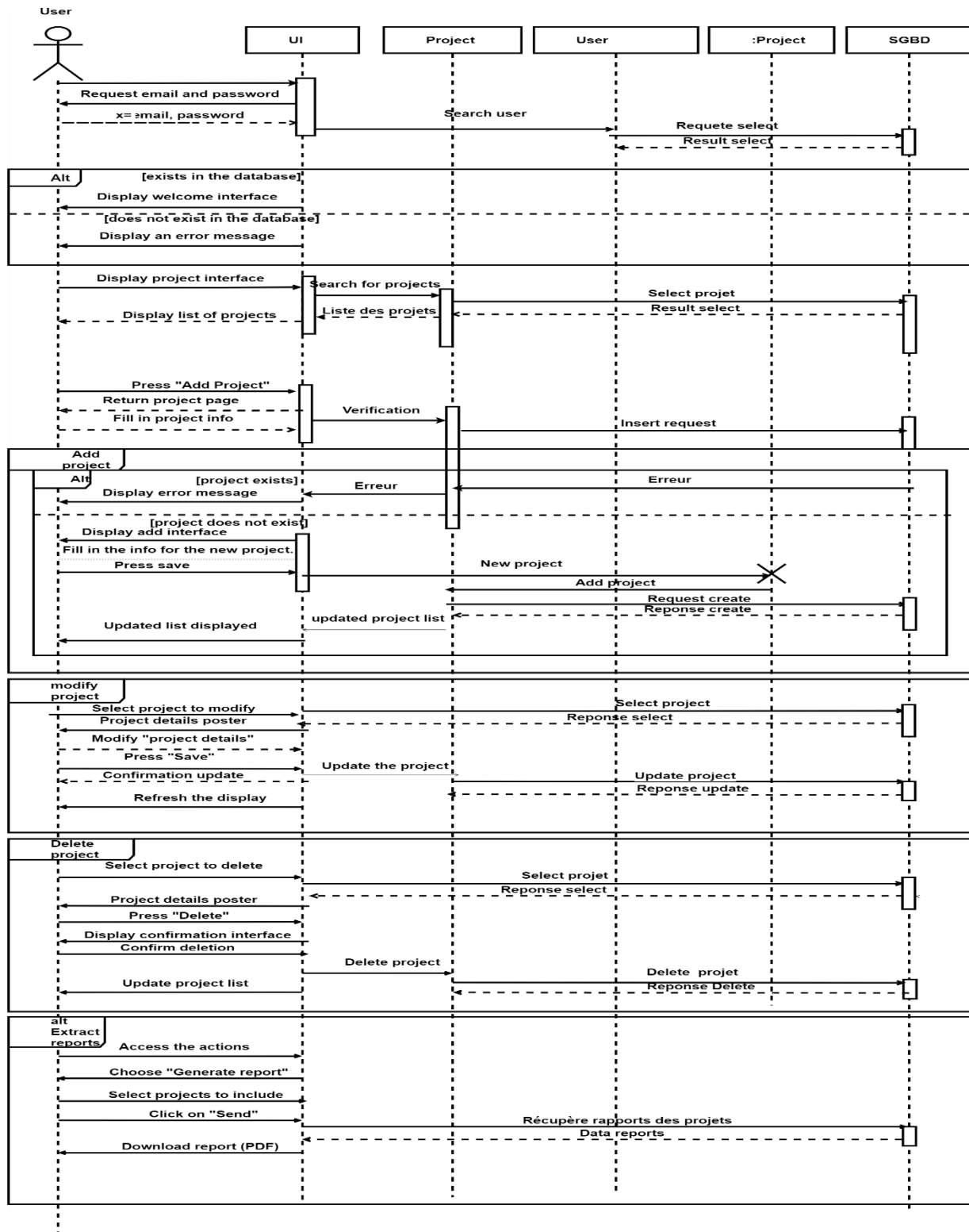
Figure 3 : Sequence diagram
