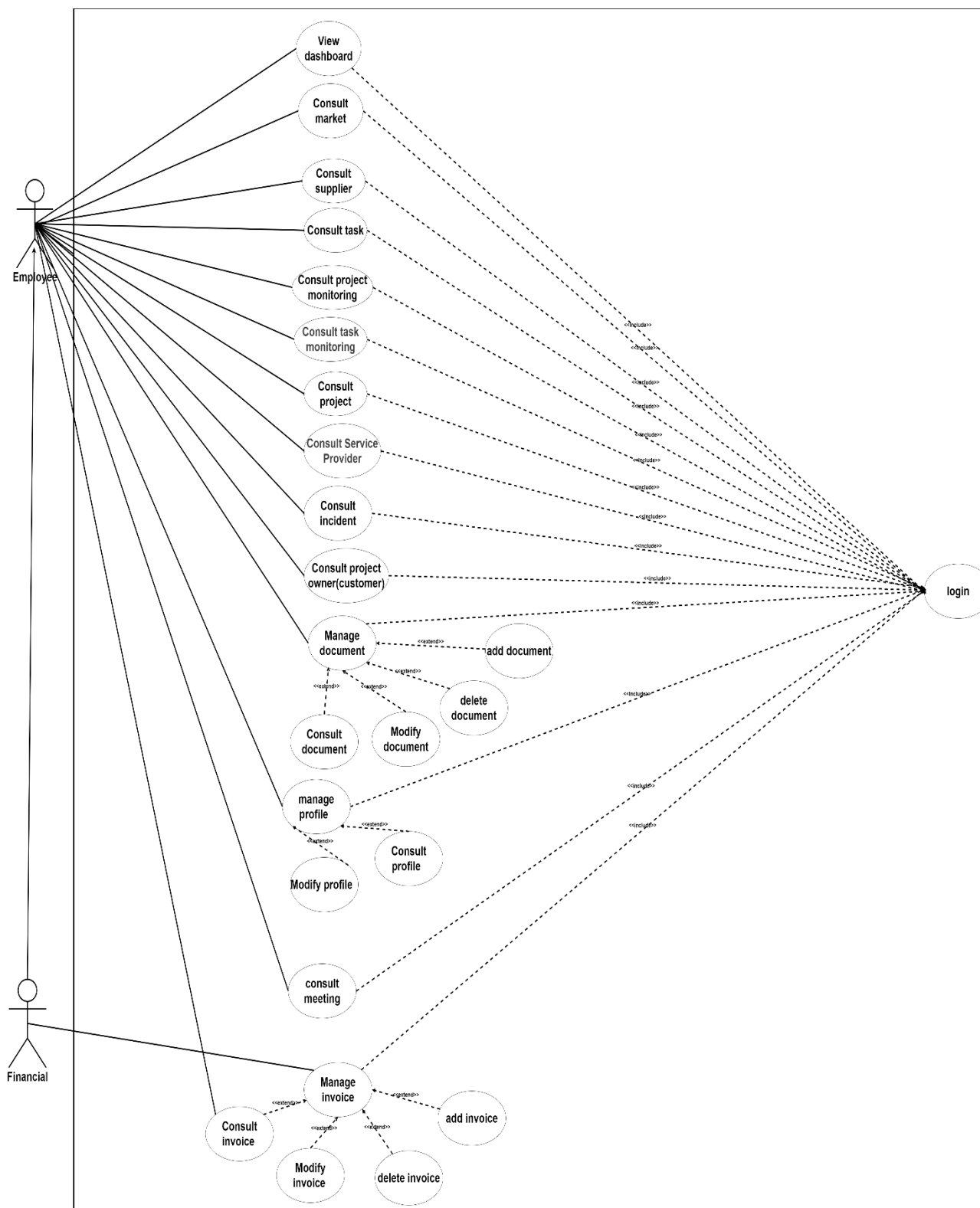
Figure 17:Employee and financier use case diagram
