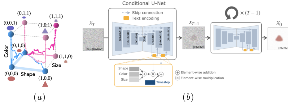
Figure S1: Model architecture and compositional task. (A) The eight combinations of three binary factors (shape, colour, size); four are used for training (blue), while four are held out at one (light pink) or two (dark pink) nodes in Hamming distance. (B) Conditional diffusion model architecture, adapted from Okawa et al. (2025). The denoising process is parameterized by a U-Net with downsampling and upsampling blocks connected by skip connections and conditioned on the target feature classes. Reproduced from Okawa et al. (2025)
