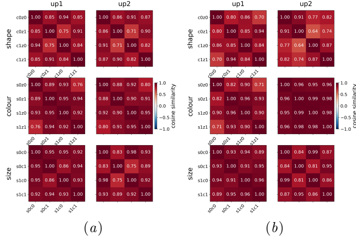
Figure S4: Context dependence of feature directions in Up1 and Up2. Pairwise cosine similarity between context-conditional feature vectors at step 1,000 (A) and step 5,000 (B). Feature representations are highly consistent across contexts at both checkpoints (most cosine similarities >0.85 ; all >0.7 except one at \sim 0.64 )
