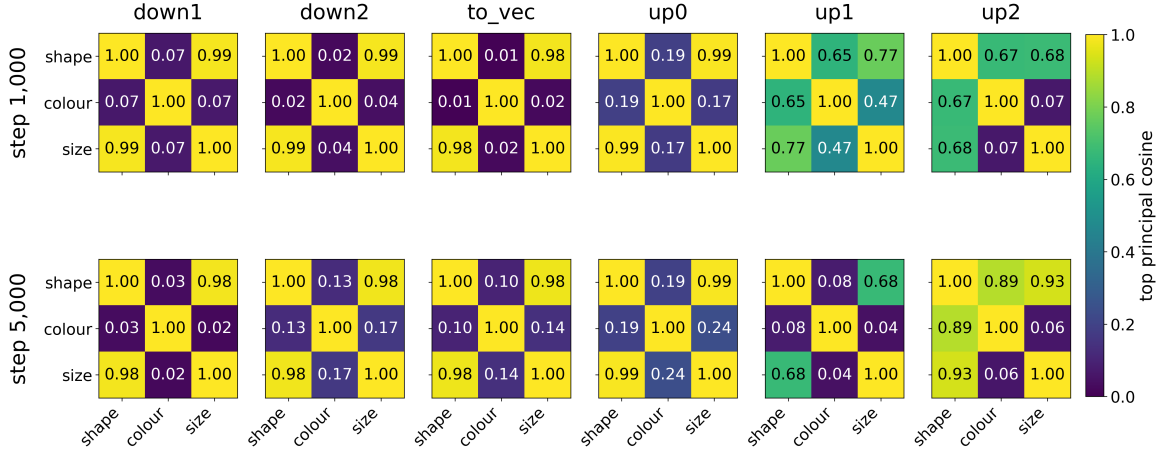
Figure 1: Feature-vector geometry before and after compositional generalization. Pairwise cosine similarity between shape, colour, and size directions at steps 1,000 and 5,000. Geometry is comparatively stable in the encoder, with the largest changes in Up1 and Up2
