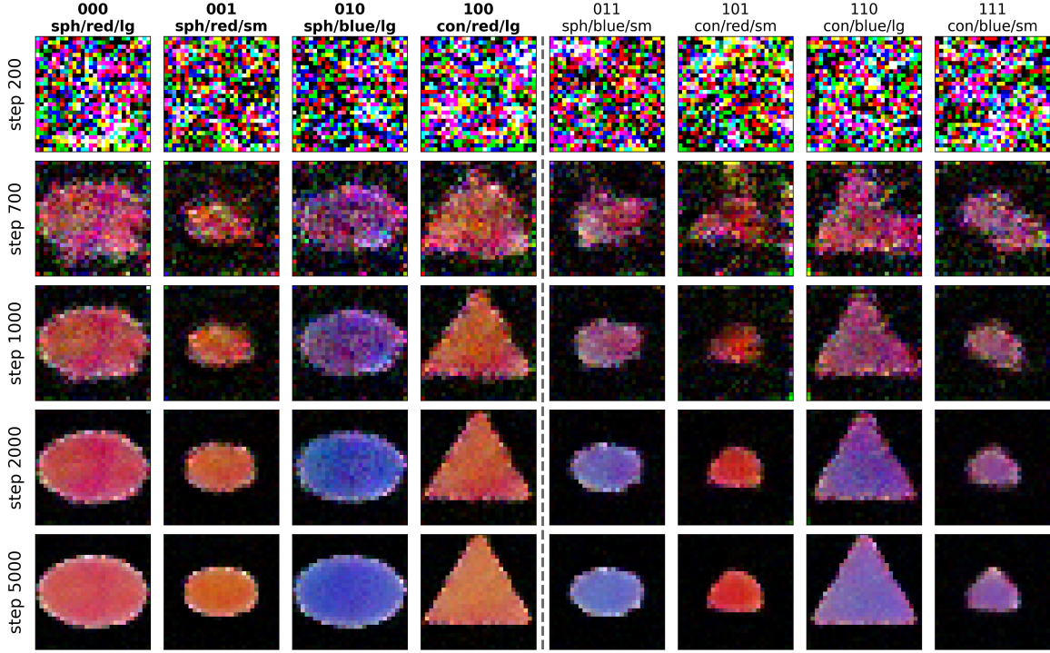
Figure S3: Generated examples throughout training. Example generations for each feature combination across training checkpoints. Samples progressively improve in fidelity to the conditioning features, from poor or incomplete compositions early in training to accurate generation of both training and held-out combinations at later checkpoints.
