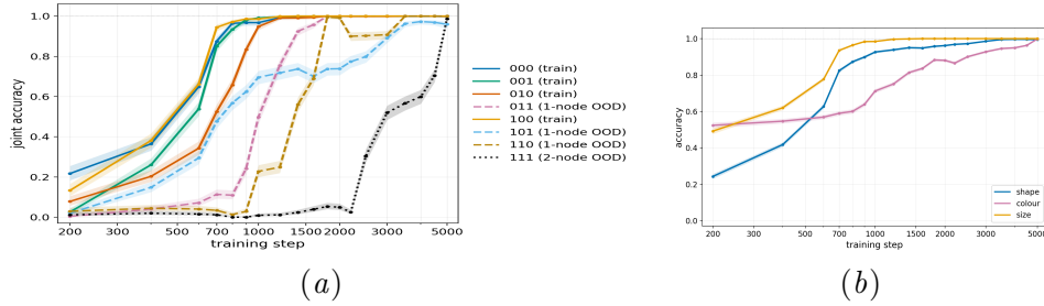
Figure S2: Emergence of compositional generalization during training. (A) Exact-combination accuracy for training and held-out combinations. The model memorizes the training set by step 1,000 and generalizes to all held-out combinations by step 5,000. (B) Feature-wise accuracy across training. Shape and size are learned earlier, while colour is the last feature to reach high accuracy.
