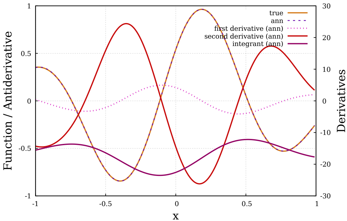
Artificial Neural Network assignment B
