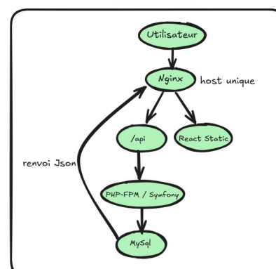
environnement production : NPM run build = compilation dossier build
