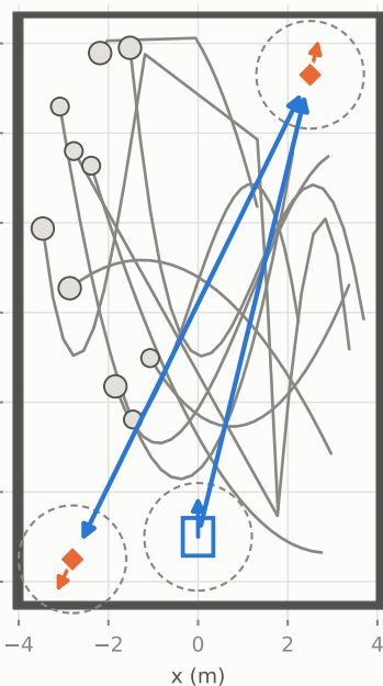
(f) dyn5: 10 obstacles peak speed 0.31–0.98 m/s
