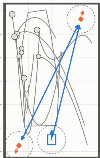
(f) dyn5: 10 obstacles peak speed 0.31–0.98 m/s
