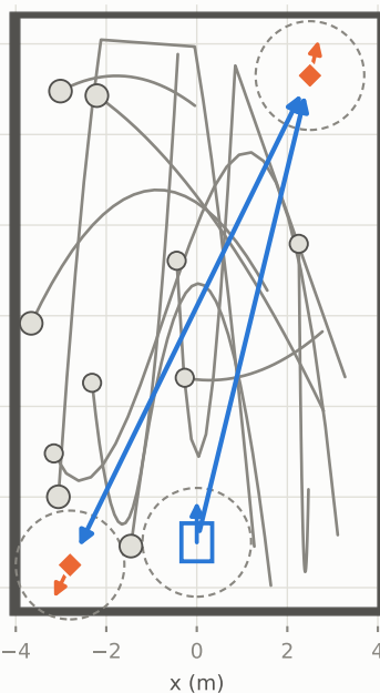
(e) dyn4: 10 obstacles peak speed 0.33–0.91 m/s
