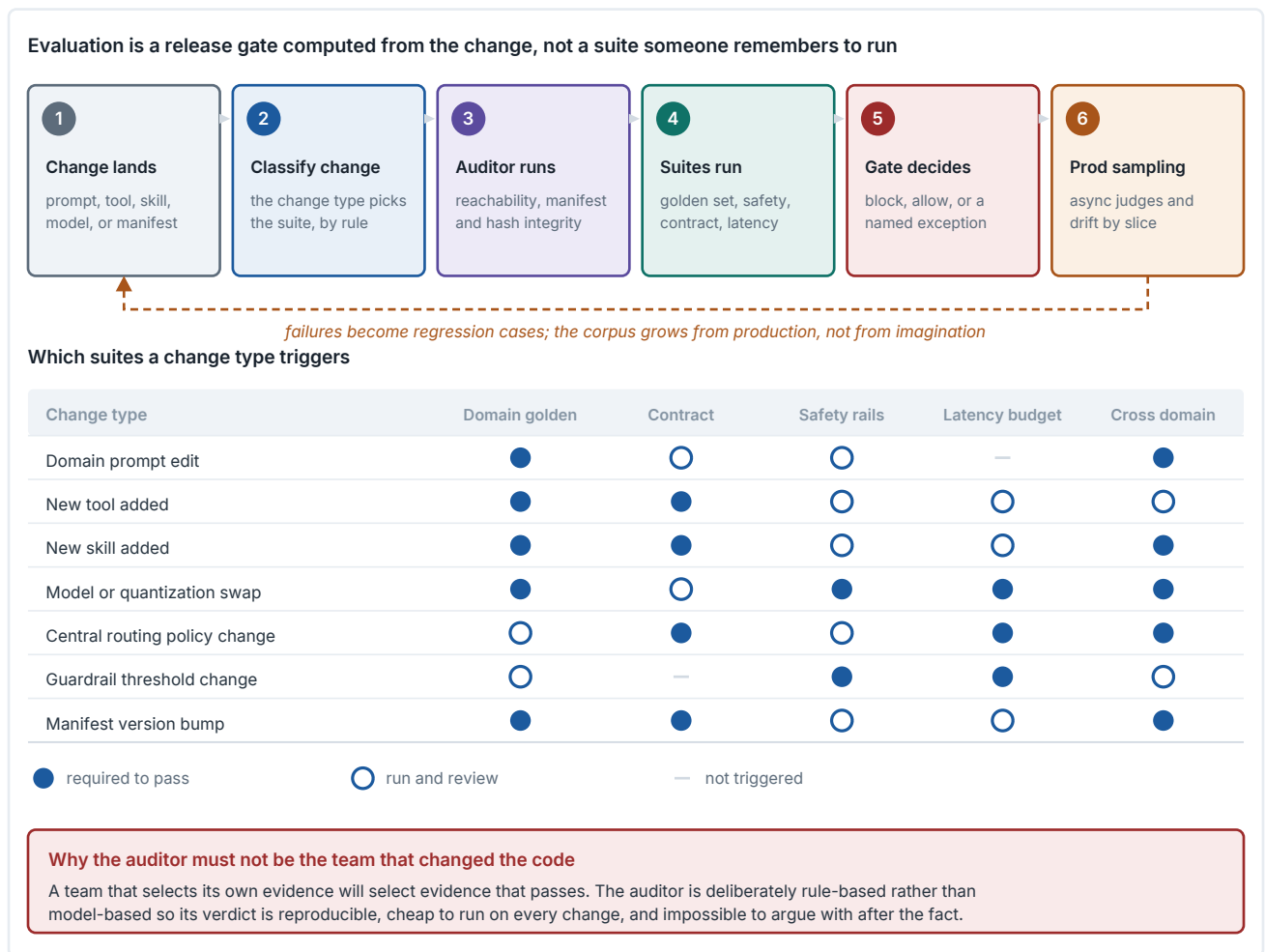
Figure 18. The evaluation lifecycle as a computed gate. The matrix in the middle is drawn from Table Table 36, which is the normative version: it maps change types to the suites they require, so that suite selection is a lookup rather than a decision made under release pressure. The closing note states why the auditor must not be the team that made the change.
