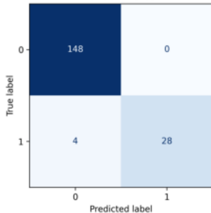
Random Forest
