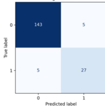
Weighted KNN
