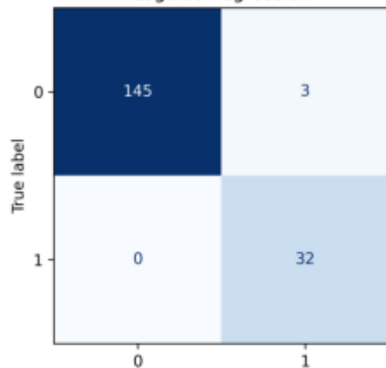
Logistic Regression
