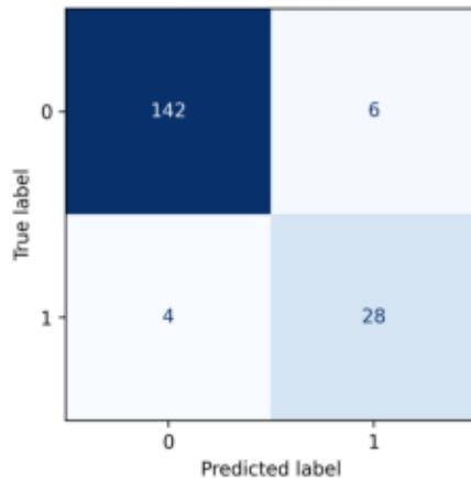
Neural Network
