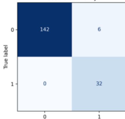
Cosine Similarity
