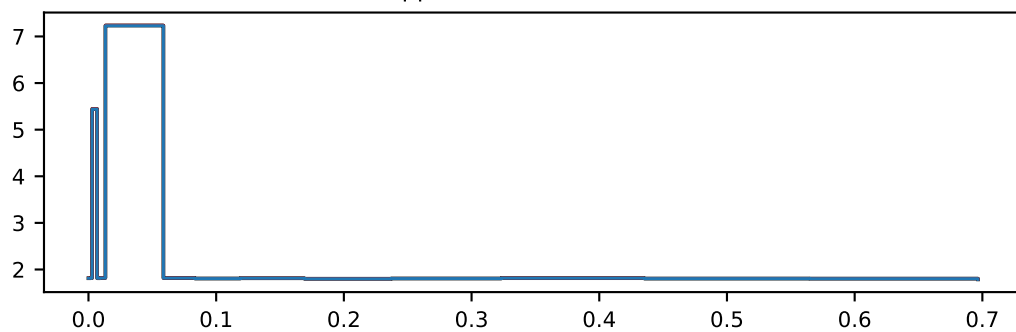
qqZZ (nom rate=36.2)
