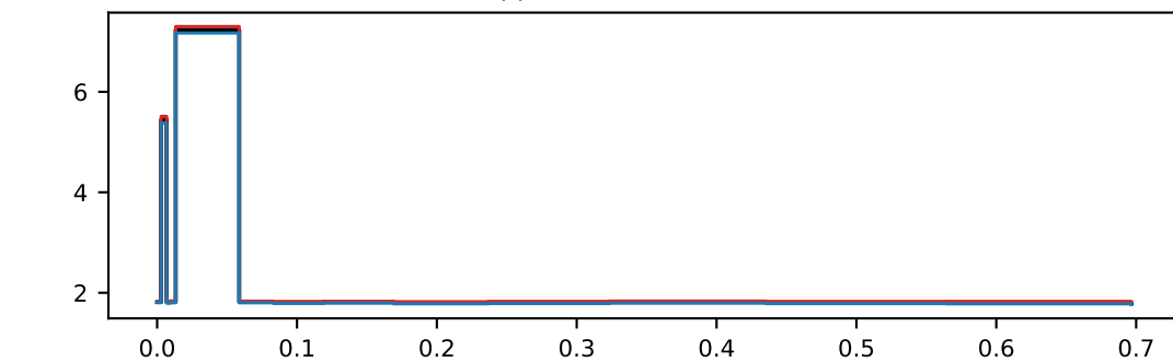
qqZZ (nom rate=36.2)
