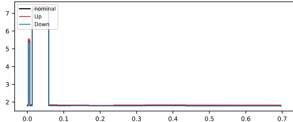
Shape systematic: scalevar_muR
