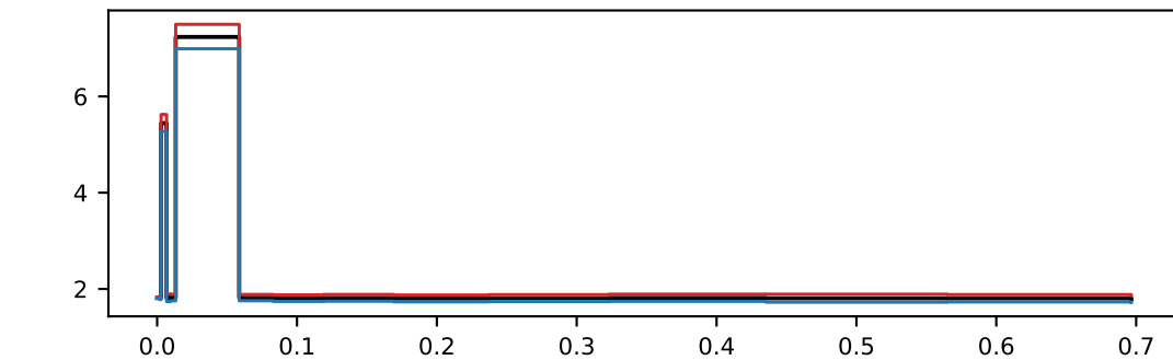
qqZZ (nom rate=36.2)
