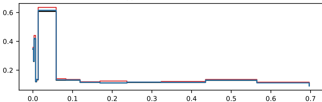
ggZZ (nom rate=2.944)
