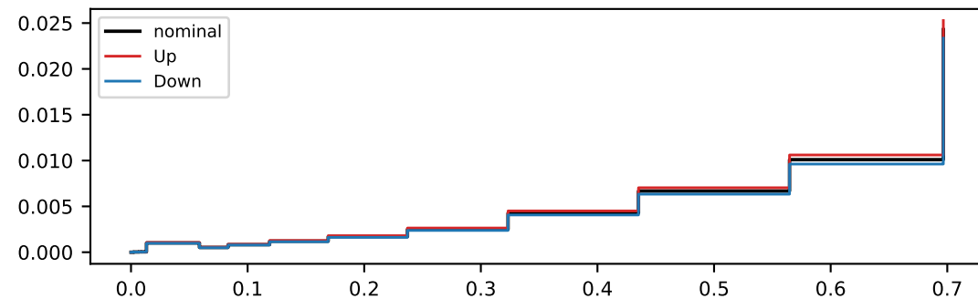
Signal (nom rate=0.05322)
