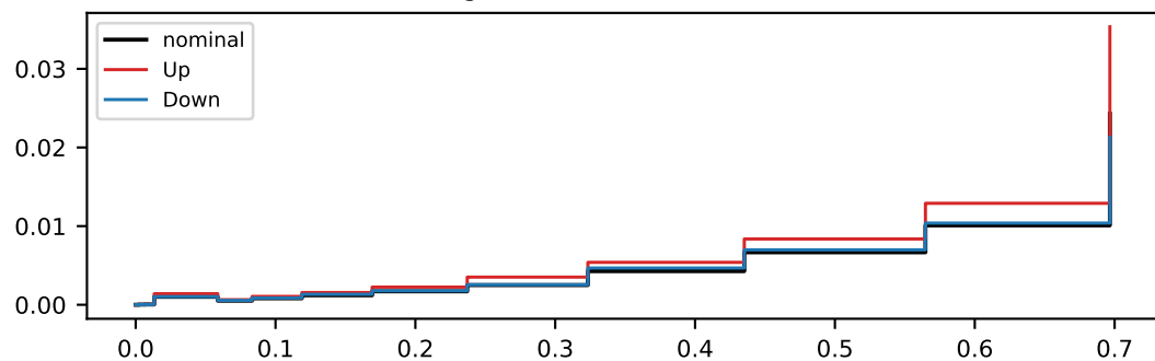
Signal (nom rate=0.05322)
