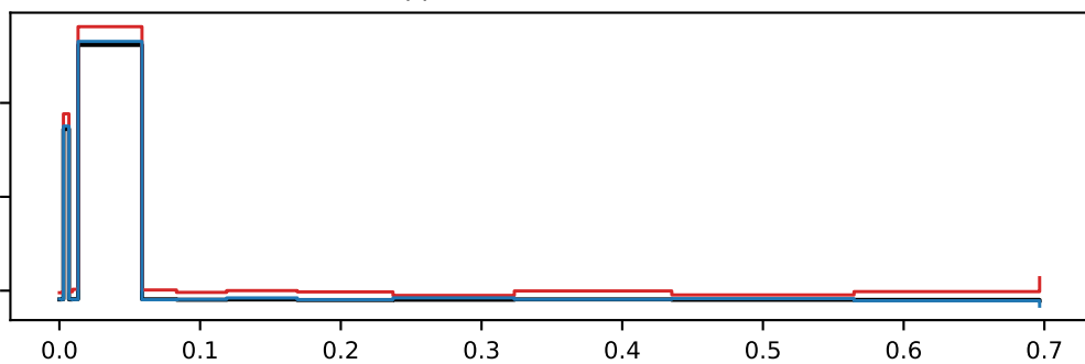
qqZZ (nom rate=36.2)
