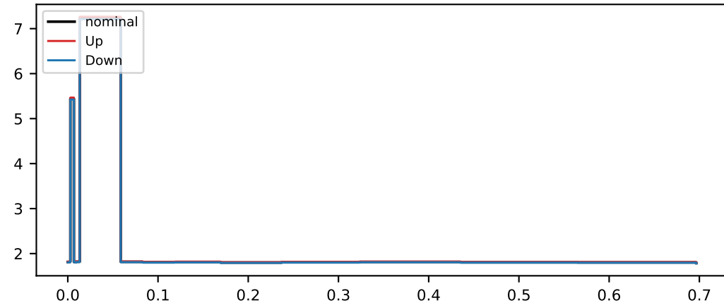
Shape systematic: lhe_pdf qqZZ (nom rate=36.2)
