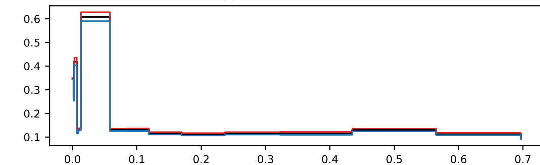
ggZZ (nom rate=2.944)
