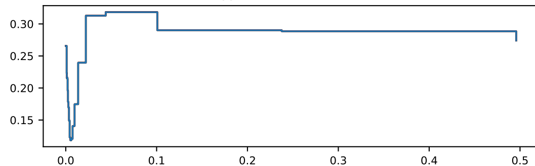
ggZZ (nom rate=4.23)
