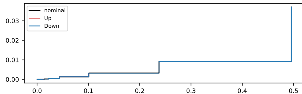
Signal (nom rate=0.05178)
