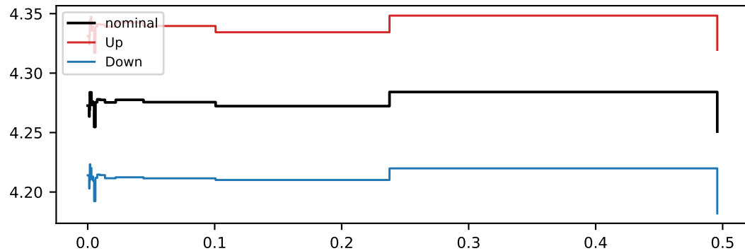
qqZZ (nom rate=85.47)
