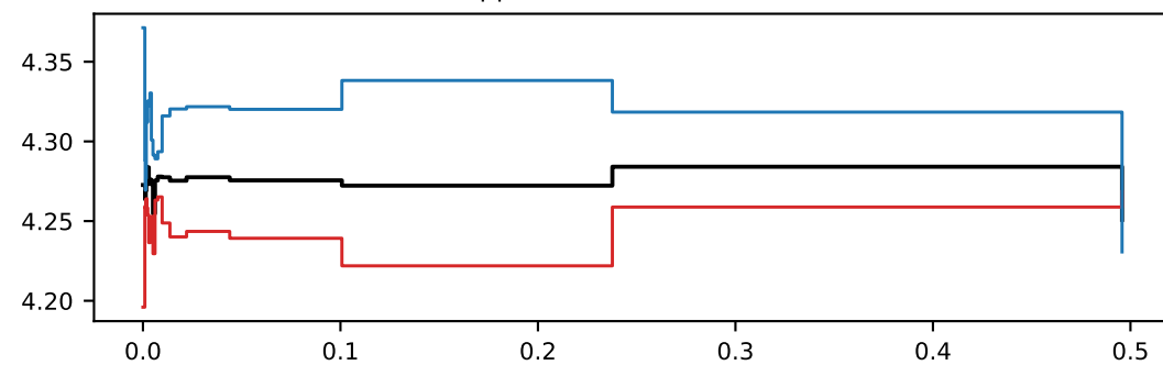
qqZZ (nom rate=85.47)
