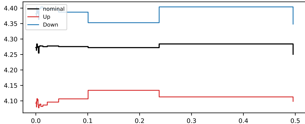
Shape systematic: scalevar_muF
