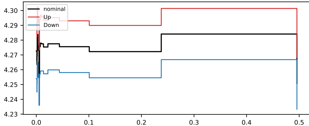
Shape systematic: lhe_pdf qqZZ (nom rate=85.47)
