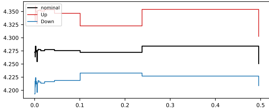
Shape systematic: scalevar_muR
