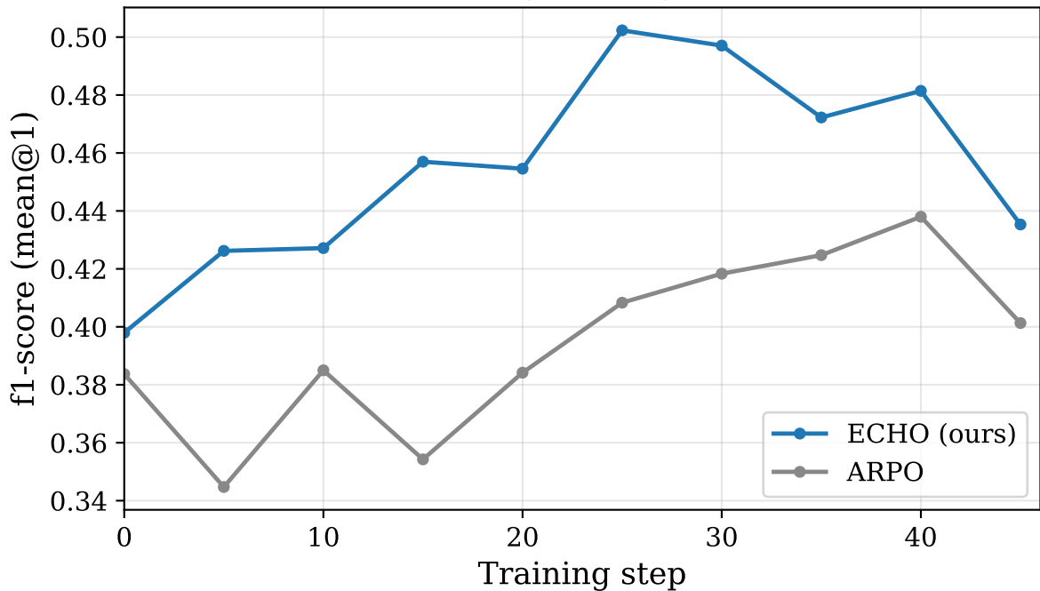
training convergence
