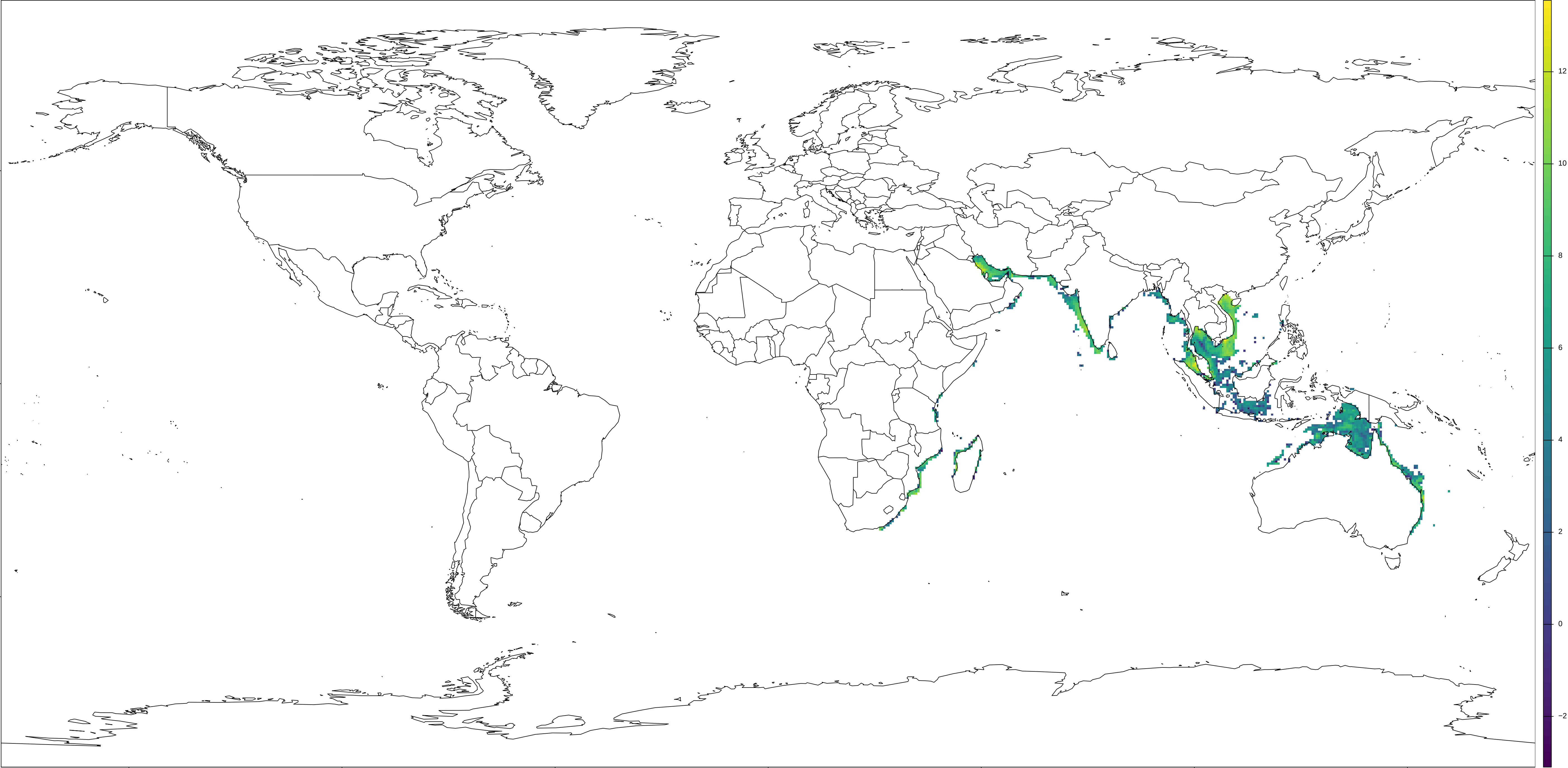
Figure 1: Summed log-scale fishing hours of Smalleye Stingray (Megatrygon microps), masked to the upper quartile of habitat suitability. The map highlights
