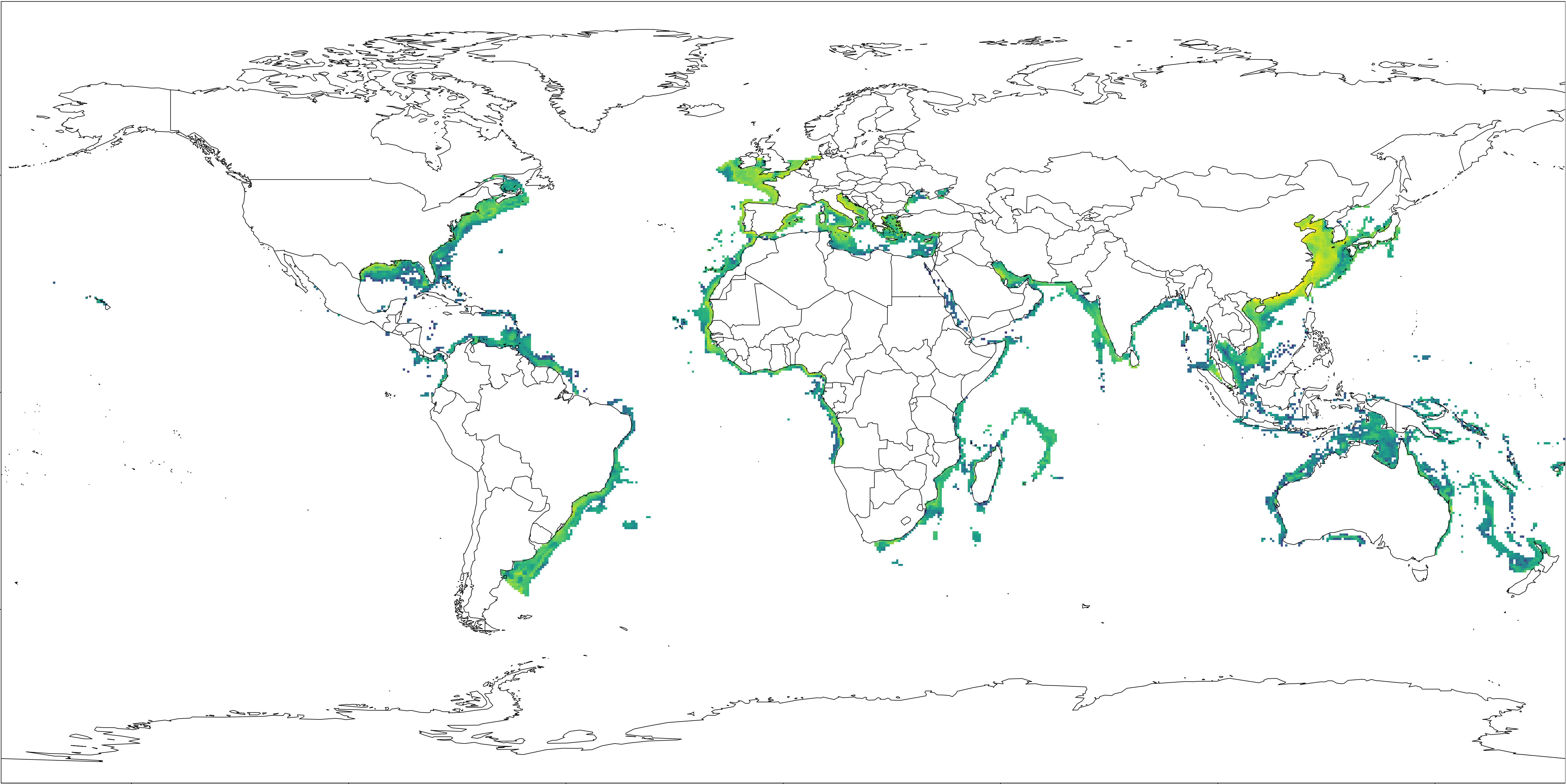
Figure 1: Summed log-scale fishing hours of Sandbar Shark ( Carcharhinus plumbeus ), masked to the upper quartile of habitat suitability. The map highlights
