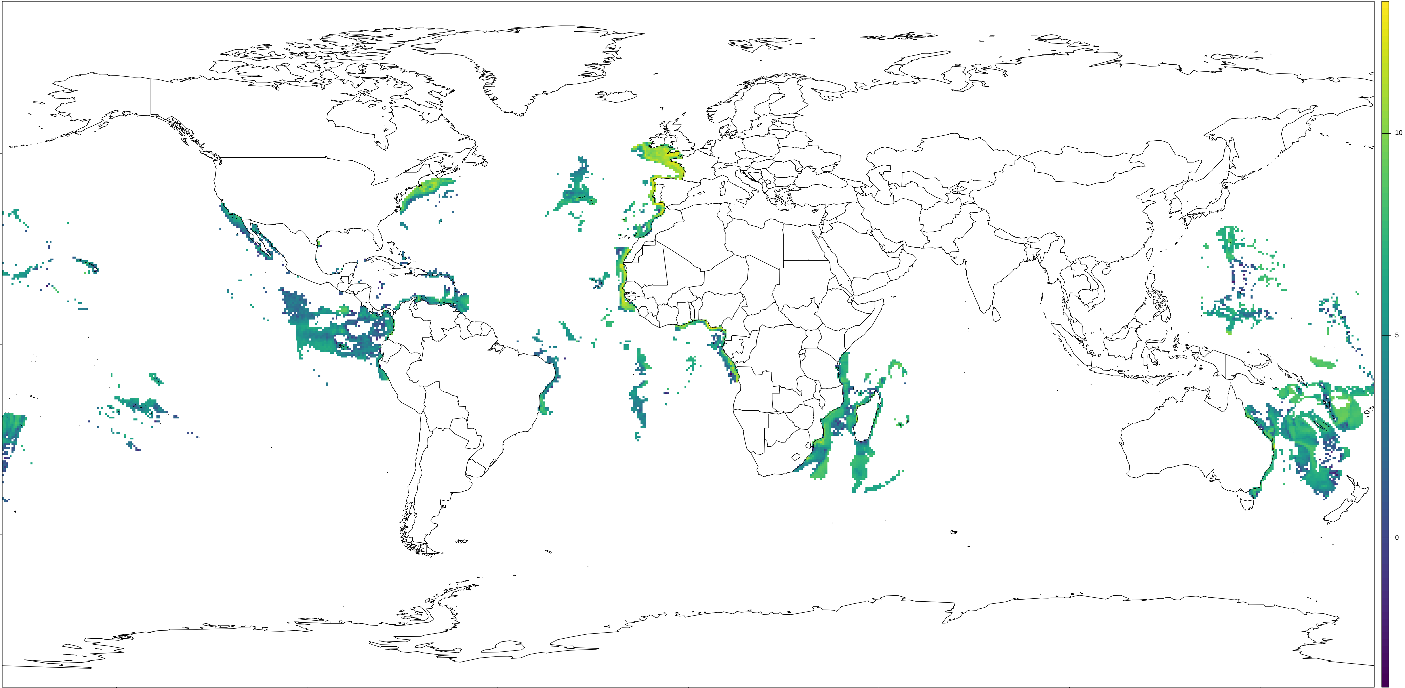
Figure 1: Summed log-scale fishing hours of Galapagos Shark Carcharhinus galapagensis , masked to the upper quartile of habitat suitability. The map highlights
