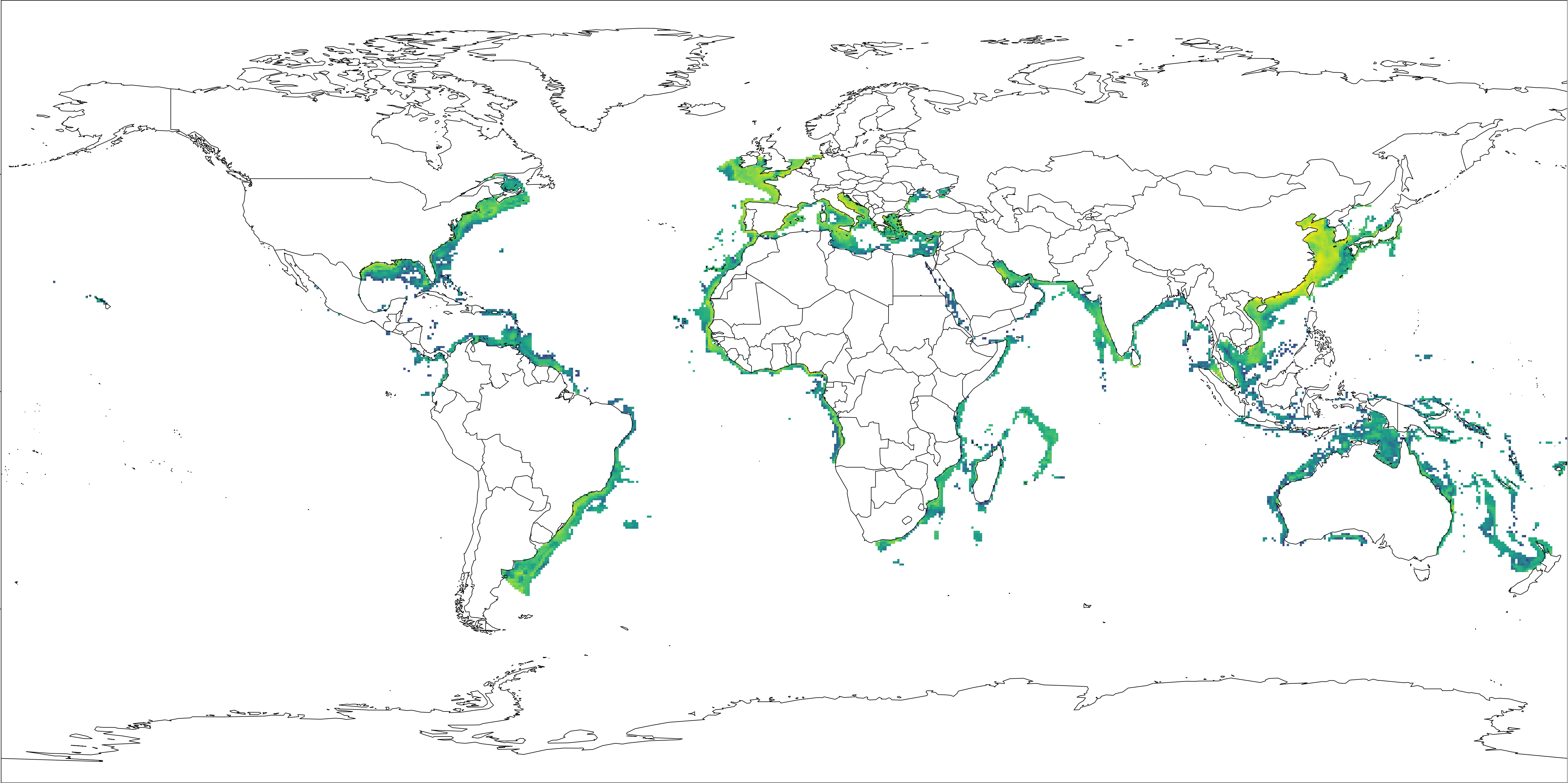
Figure 3: Summed log-scale fishing hours of Sandbar shark ( Carcharhinus plumbeus ), masked to the upper quartile of habitat suitability. The map highlights areas the species is most impacted by the following gears: drifting-longlines, pole-and-line, set-gillnets, set-longlines, trawlers.
