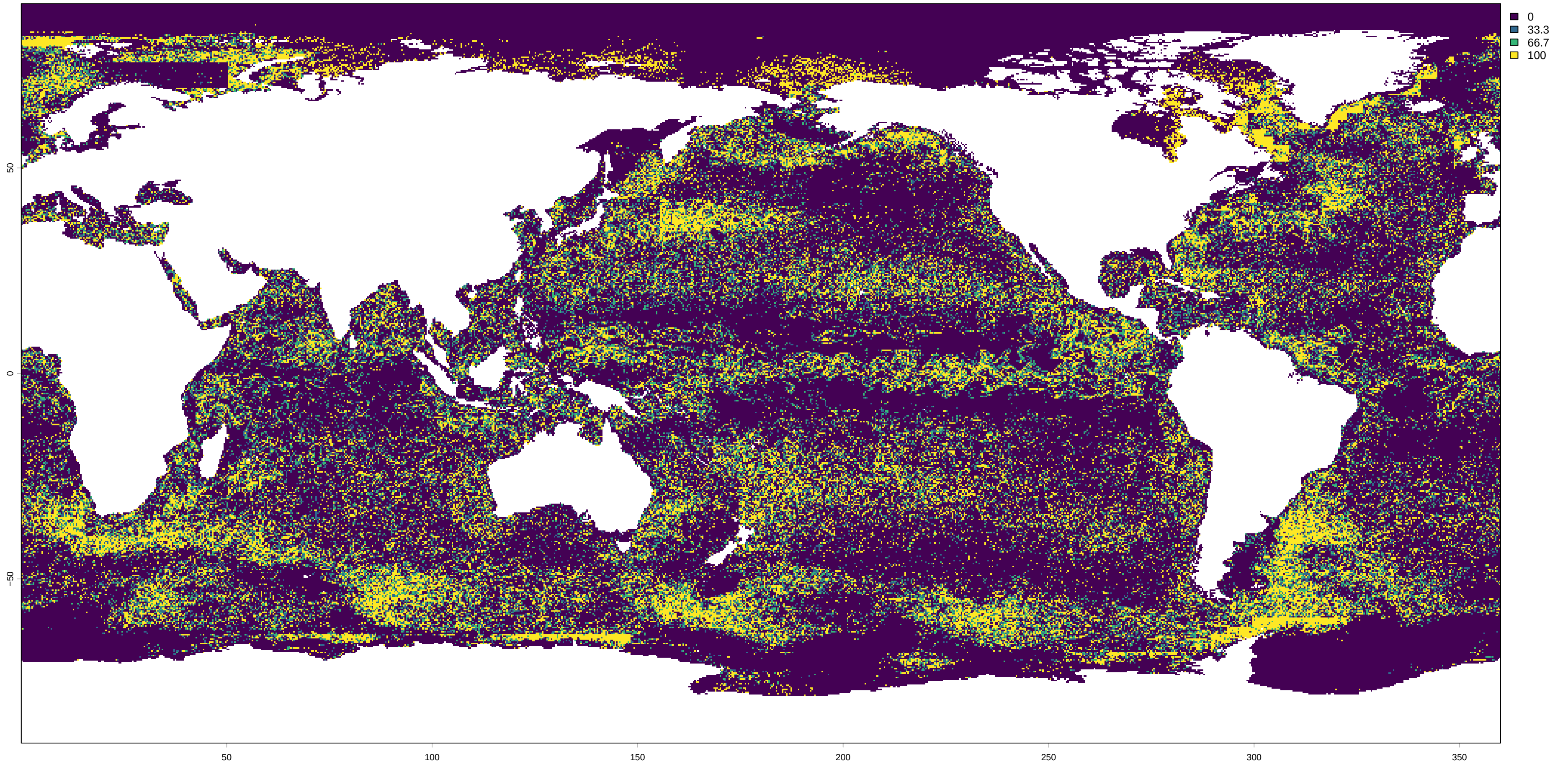
Longhurst-relative Q3 persistence (%) – 2 days
