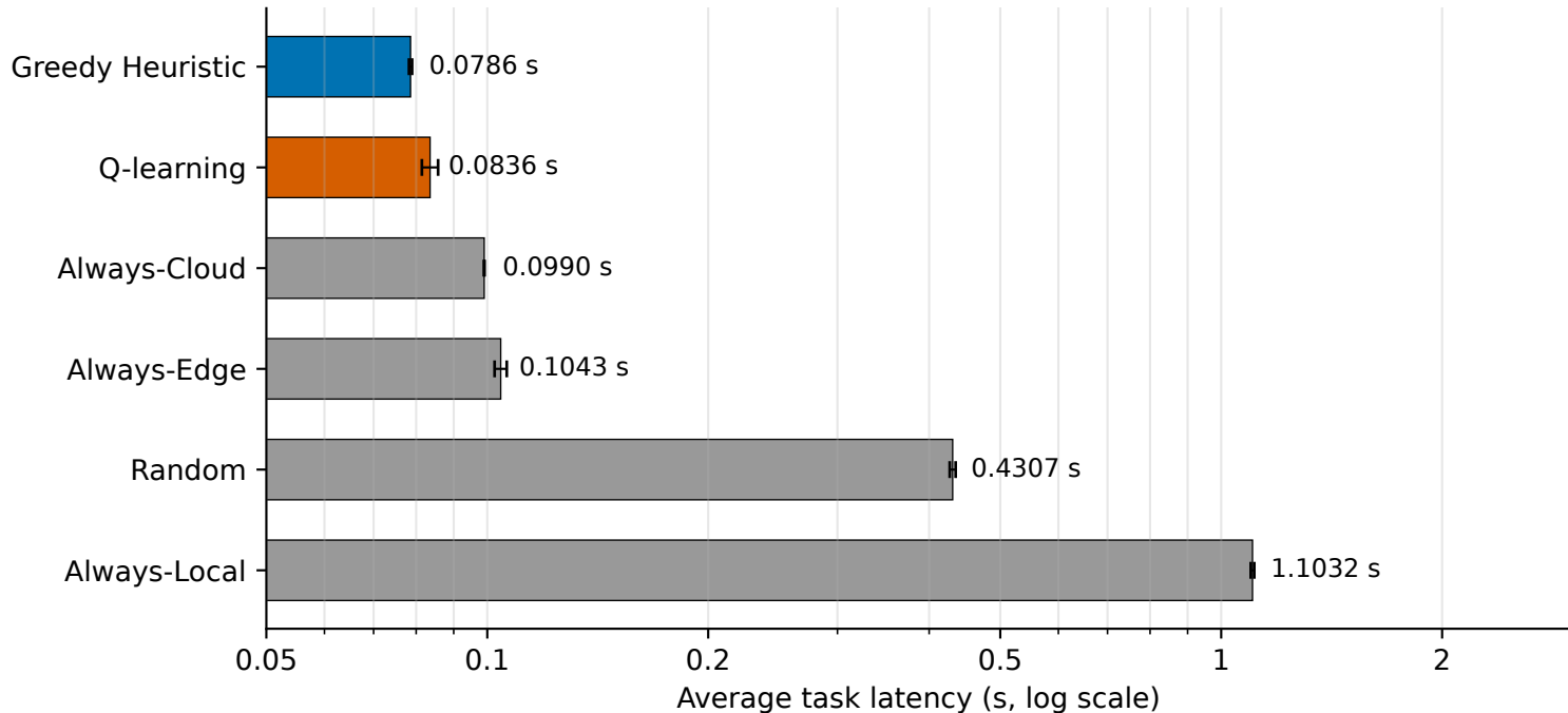
Average task latency by strategy (mean of 5 seeds, 95% CI)
