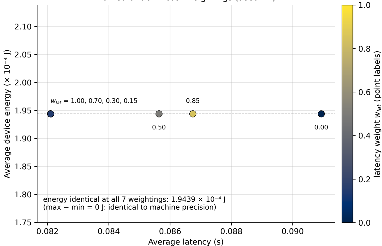
Latency-energy operating points of Q-learning agents trained under 7 cost weightings (seed 42)
