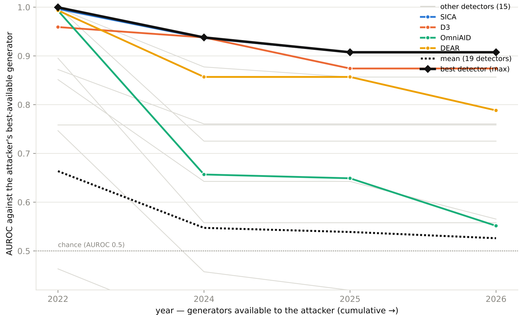
Attacker picks the best generator: detector AUROC over time
