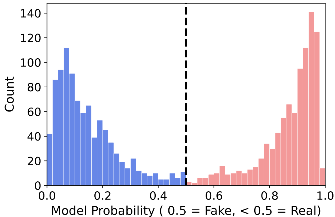
Before PGD Attack
