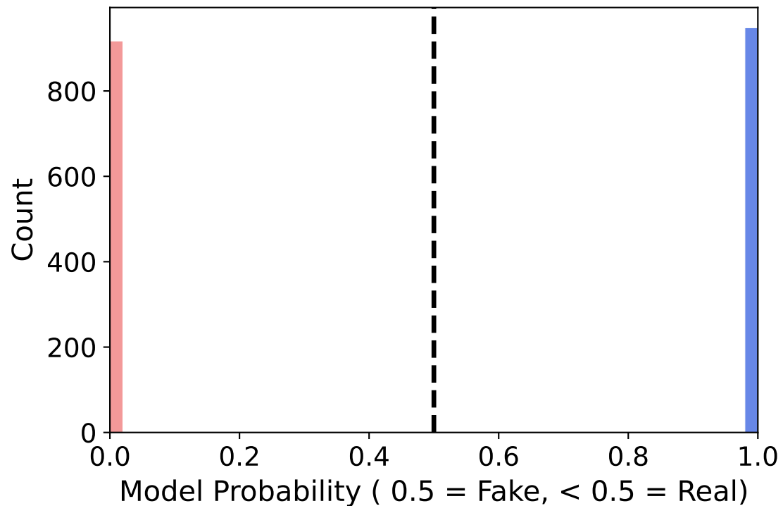
After PGD Attack
