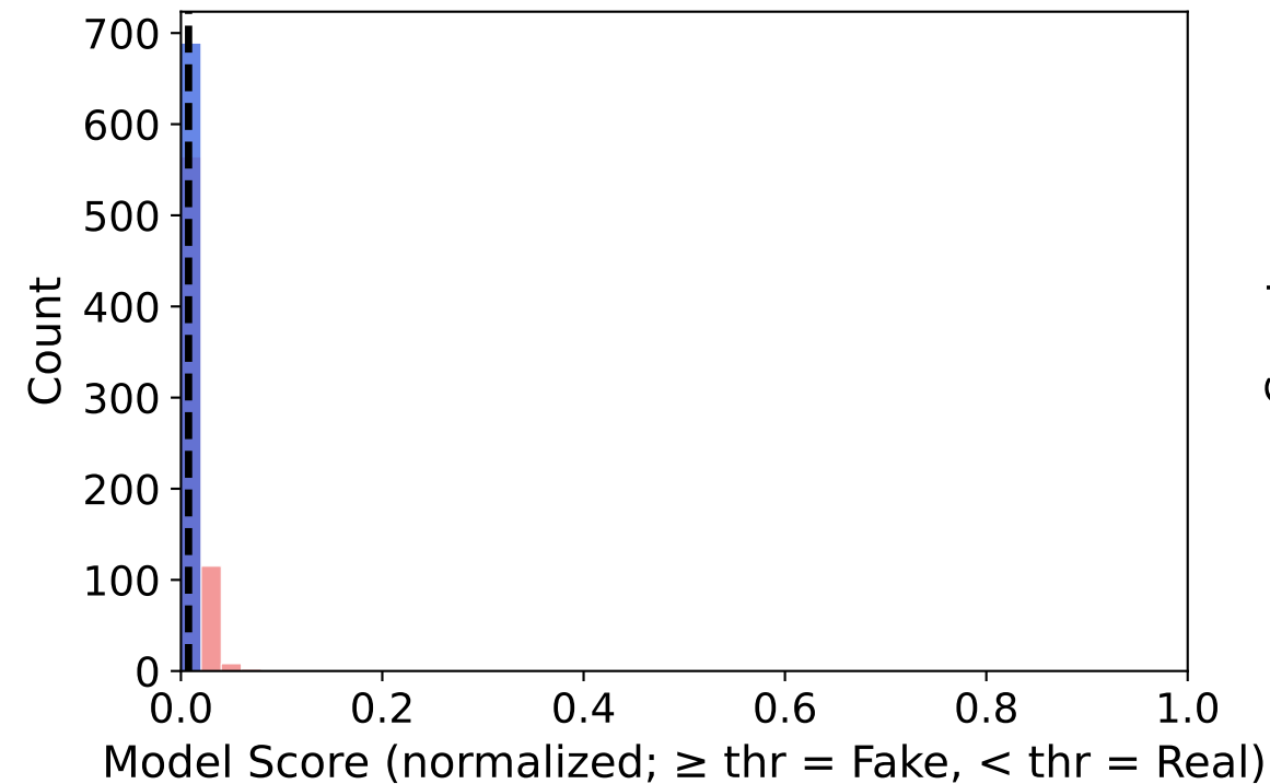
Before PGD Attack
