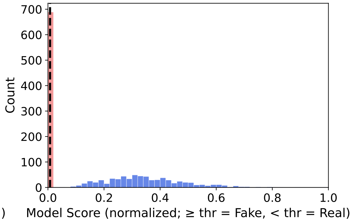
After PGD Attack
