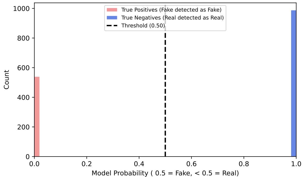
After PGD Attack
