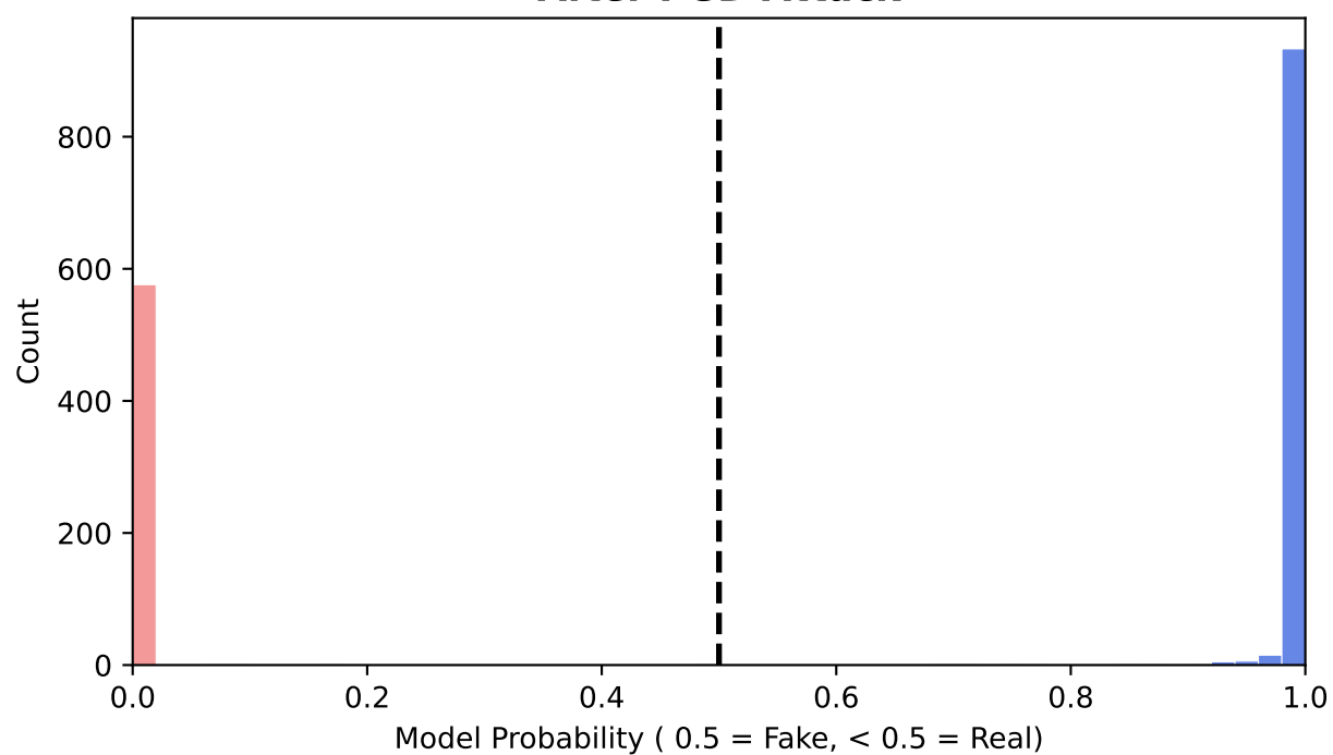
After PGD Attack
