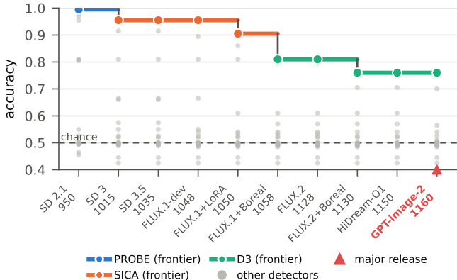
Detection accuracy vs. generator Elo
