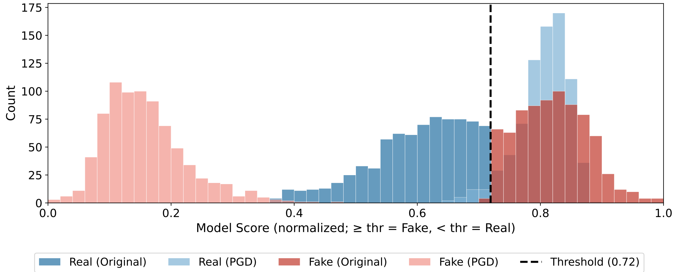
AEROBLADE: Prediction Scores Before vs. After PGD
