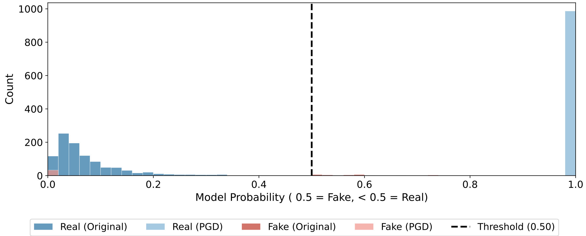
AllPatchesMatter: Prediction Scores Before vs. After PGD
