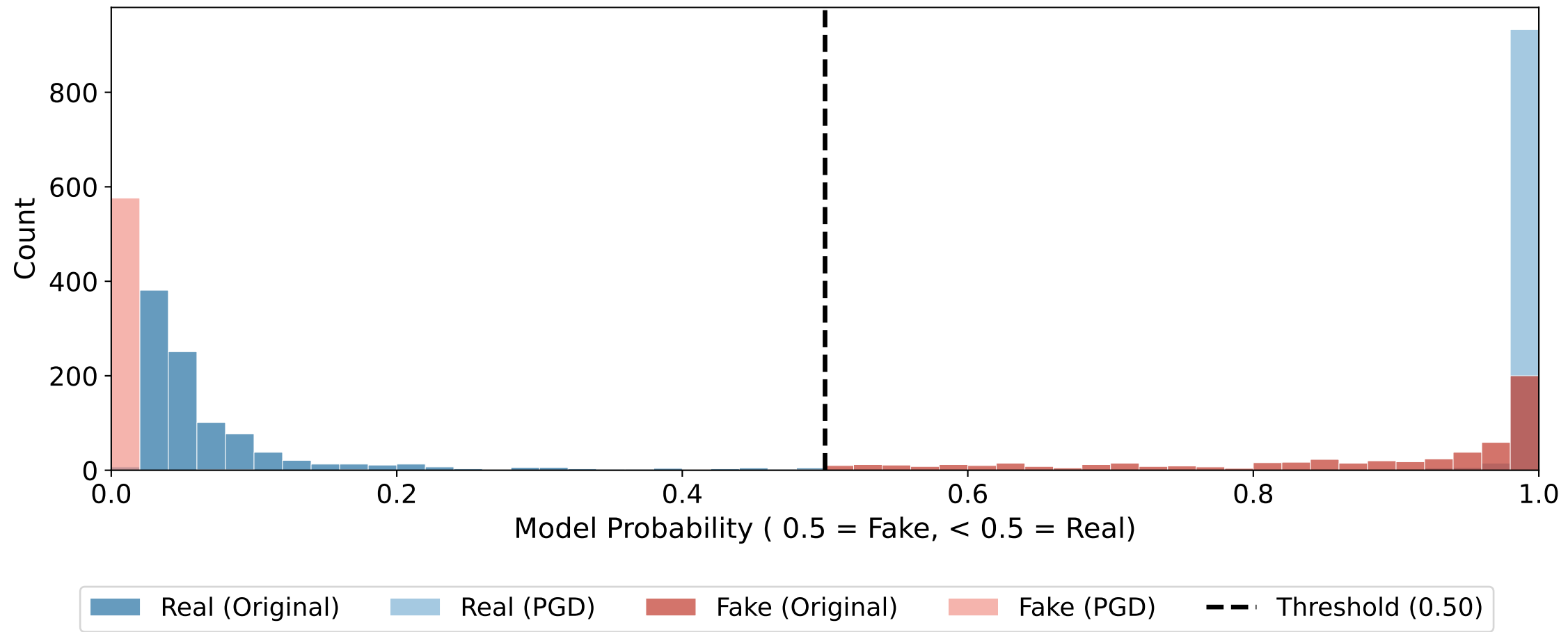
DDA: Prediction Scores Before vs. After PGD
