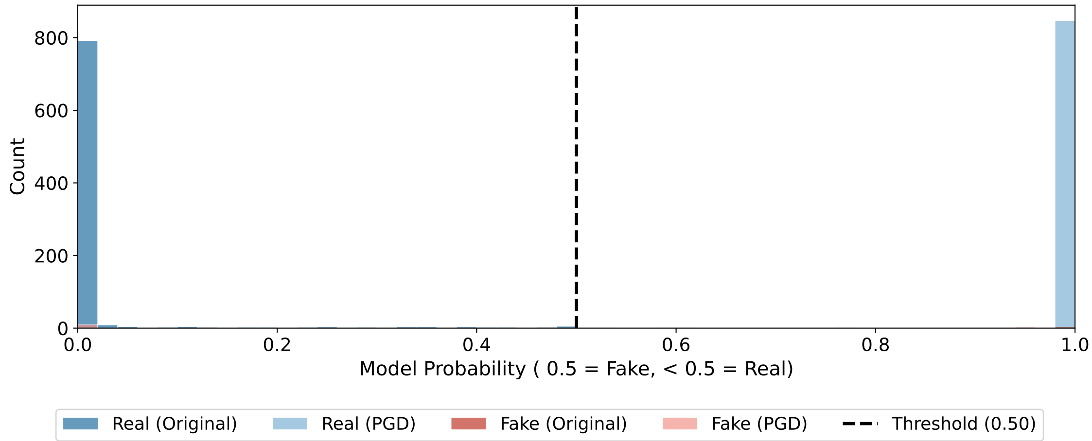
DGS-Net: Prediction Scores Before vs. After PGD
