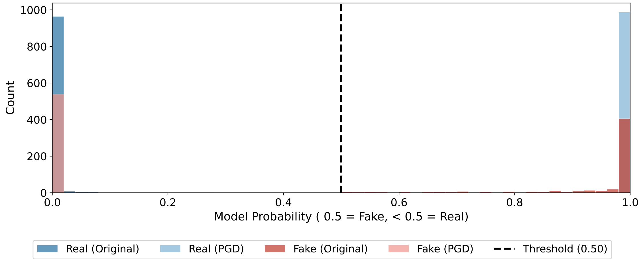
PROBE: Prediction Scores Before vs. After PGD
