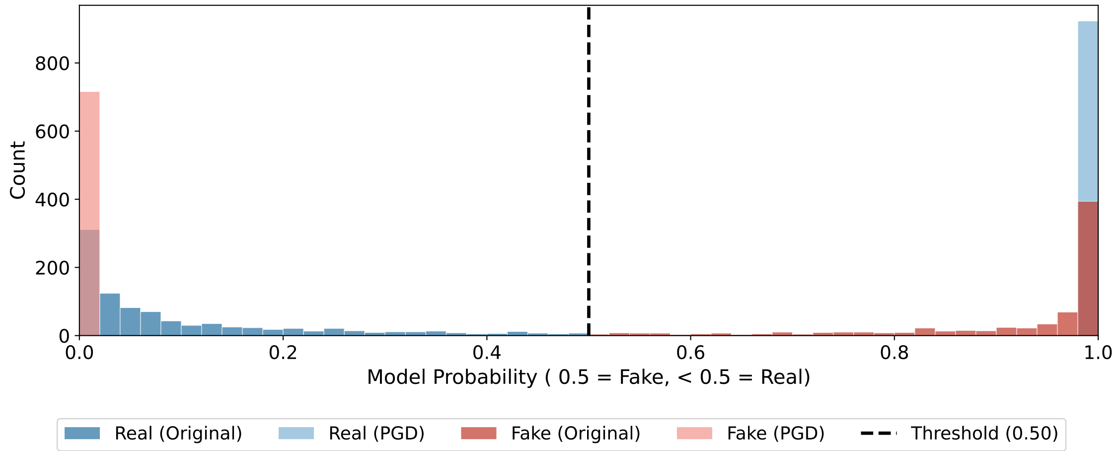
SICA: Prediction Scores Before vs. After PGD
