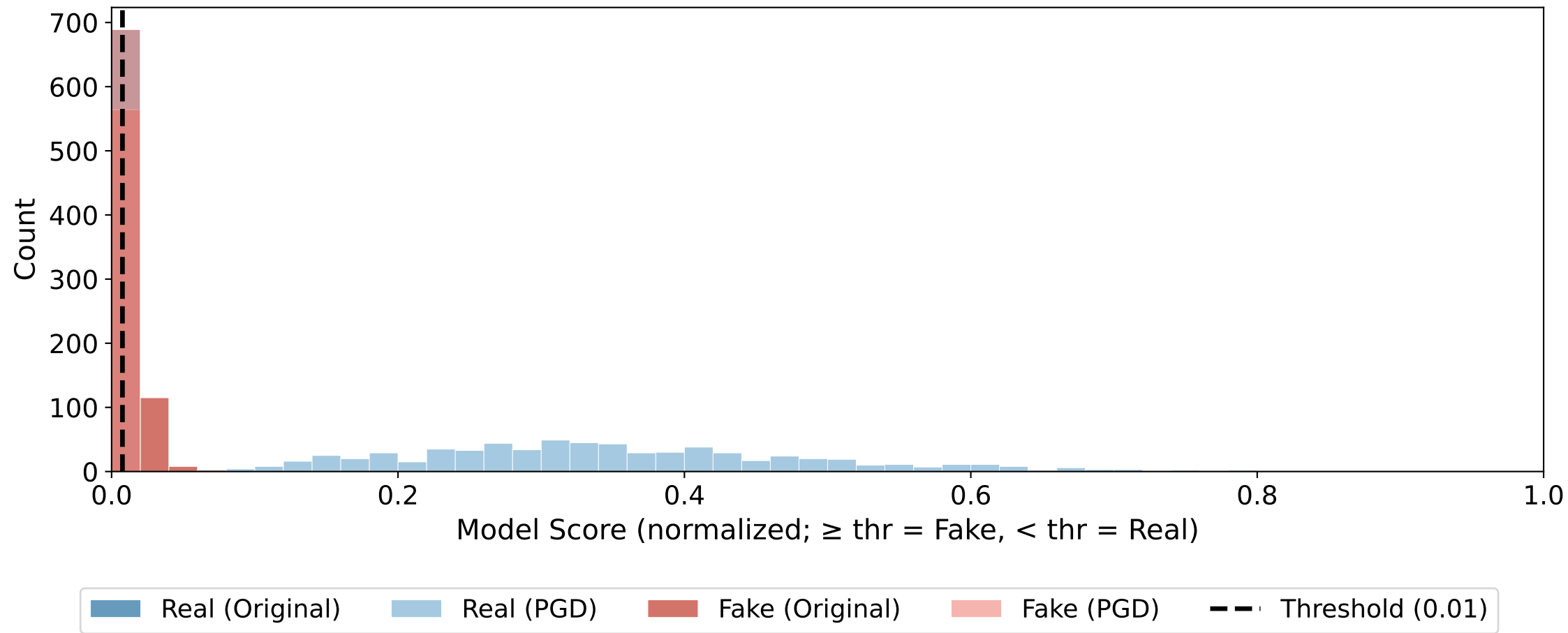
WaRPAD: Prediction Scores Before vs. After PGD
