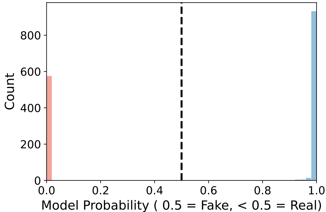
After PGD
