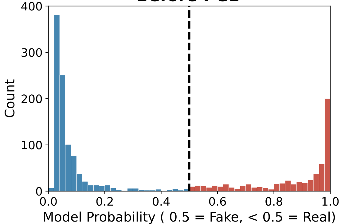
Before PGD
